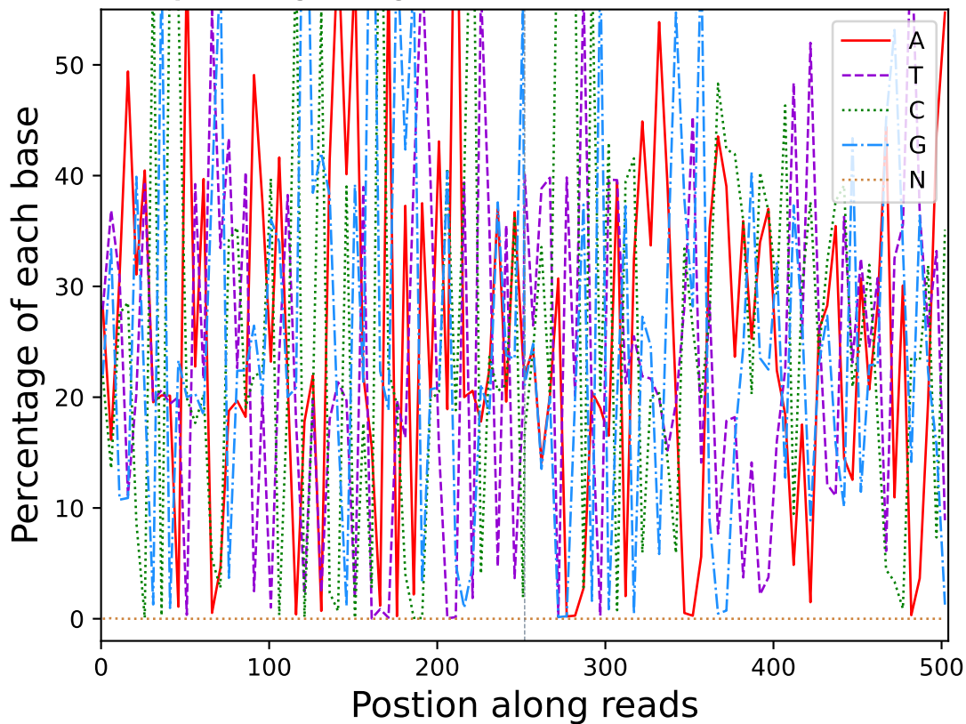
Base percentage along reads (R10407)
